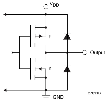
Figure 11. Equivalent Digital Output Circuit
