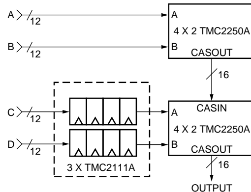
Figure 12. Performing Cubic Convolution with Two TMC2250A's
