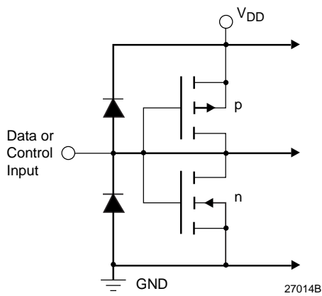
Figure 10. Equivalent Digital Input Circuit
